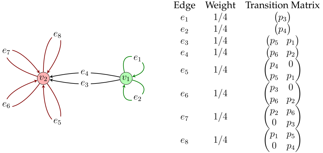
FIGURE 2. Transition graph for the Testud IFS
