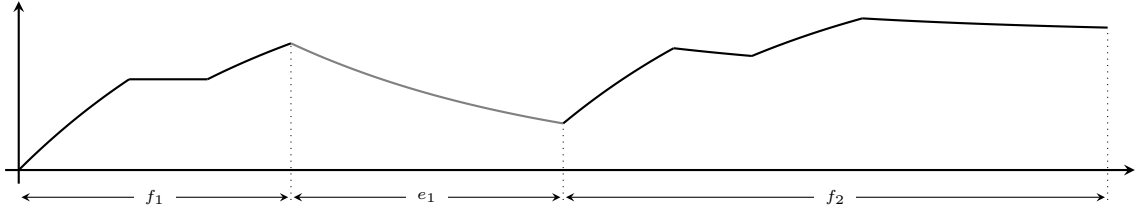
FIGURE 2. The concatenation of (f_1, e_1, f_2) corresponding to a function \phi \in \mathcal{C}_d defined in §3.3 restricted to the domain (0, \infty) .
